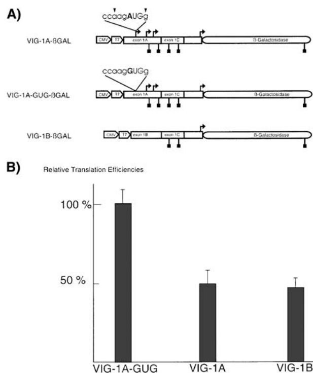
Figure 5. Disruption of the ORF in the 5' region of a vigilin splice variant results in enhanced vigilin translation as demonstrated in cell culture. (A) Schematic representation of the VIG-1A-βGal, VIG-1A-GUG-βGal and VIG-1B-βGal expression cassettes. Start and stop codons are shown as in figure 3, promoters and sequences as in figure 4. The authentic vigilin start codon in exon 2 is used to drive expression of the \beta -galactosidase reporter gene. (B) Translation efficiencies of the VIG-1A, VIG-1A-GUG and VIG-1B leader sequence-βGal fusions. Bars represent the mean \pm SEM of three independent transfection experiments in CV1 cells.
