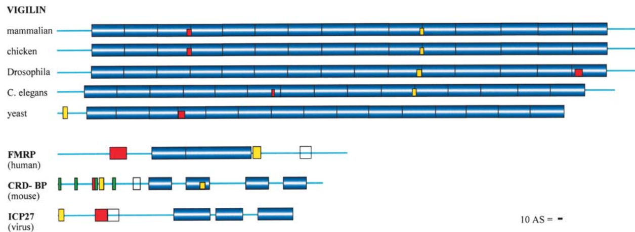
Figure 2. Vigilins represent a unique family among KH proteins. Representative members of the KH protein family are shown including vigilins from different organisms, the human fragile X mental retardation protein (FMRP), the mouse coding-region-determinant-binding protein (CRD-BP) and the herpes-simplex-virus-infected cell polypeptide 27 (ICP27). Homology domains are indicated. Because of the high similarity between mouse, rat and human vigilin they are presented as the mammalian vigilin. Boxes: blue, KH domain; red, NLS; yellow, NES; white, RGG-motif; green, ribonucleoprotein motif.
