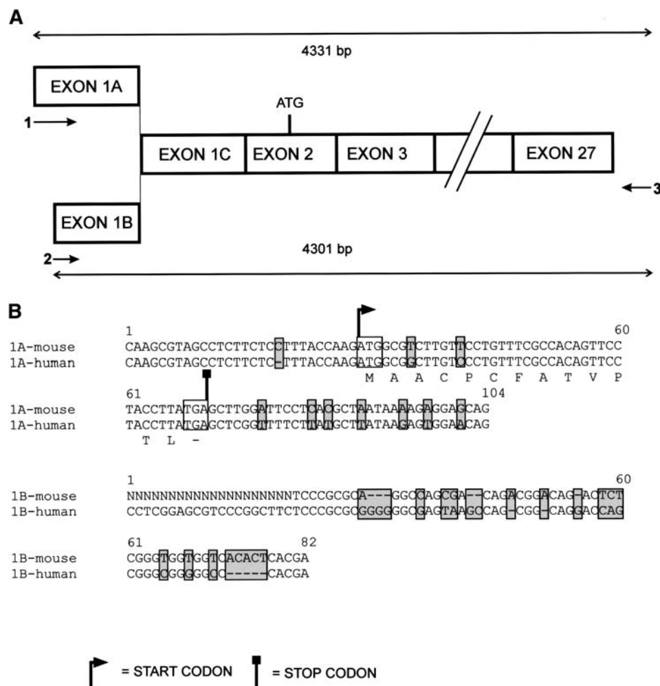
Figure 3. A conserved ORF in the 5' region of the vigilin splice variant 1A. Schematic representation demonstrating that vigilin exons 1A and 1B are alternatively spliced to exon 1C followed by exon 2 that contains the translation start codon ATG for the ORF encoding the vigilin protein (A). Alignment of the sequences of the exon 1A and 1B splice variants from mouse and human vigilin genes demonstrating that an ORF detected in exon 1A is highly conserved between mouse and human (B). Sequence differences are boxed. Arrows indicate the location of oligonucleotide primers used for cloning (exon 1A primer, 1, 3; exon 1B primer, 2, 3). The sequence of the primer binding site in exon 1A was corrected according to a published EST sequence (GenBank/EMBL/DDBJ accession no. BG077807) and is not known (N) in exon 1B.
