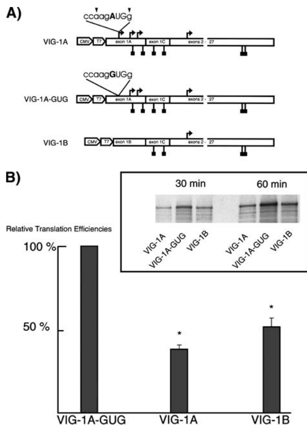
Figure 4. Disruption of the ORF in the 5' region of a vigilin splice variant results in enhanced vigilin translation as demonstrated in a cell-free system. (A) Schematic representation of the VIG-1A, VIG-1A-GUG and VIG-1B expression cassettes. Start and stop codons are shown as in figure 3. The nucleotide sequence next to the first AUG in the native VIG-1A mRNA and the mutated sequence in the VIG-1A-GUG transcript are shown in detail. Arrowheads indicate the nucleotides most important for a strong initiation potential (Kozak sequence). CMV, cytomegalovirus promoter; T7, T7 RNA polymerase promoter. (B) Translation efficiencies of the cognate VIG-1A and VIG-1B transcripts compared to the mutated VIG-1A-GUG transcripts. Bars represent the mean \pm SEM of six translation experiments. Asterisks indicate that the amounts of protein translated from the VIG-1A and VIG-1B transcripts, are statistically significantly different ( p = 0.05 ) from VIG-1A-GUG. The inset shows the fluorography of 35 S-methionine-labeled protein bands synthesized from the different transcripts.
